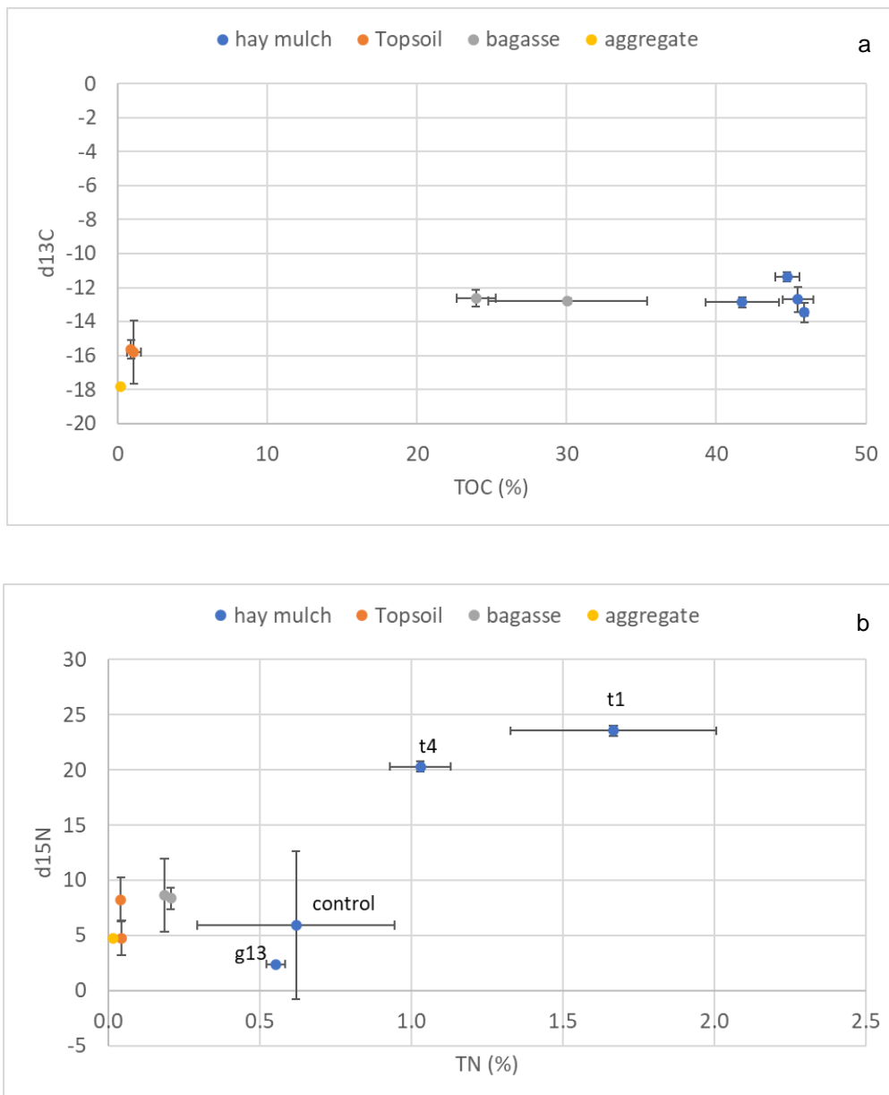
Figure 24 Mean organic carbon and d13C (a) and elemental nitrogen and d15N (b) in potential sources of particulate nutrient export in runoff after gully remediation at Strathalbyn Station. Error bars represent standard deviations of three replicates.
